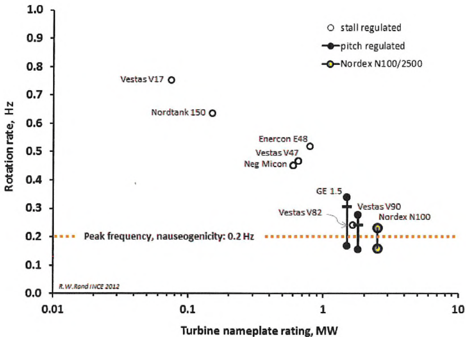
Figure 2. Chart of wind turbine rotation rates (Hz) for various wind turbine models including the Nordex N100. Note nauseogenicity range is 0.1 to 1 Hz with peak potential noted at 0.2 Hz. Note bars on GE 1.5 and Vestas V90 models indicate nominal rotation rate.
