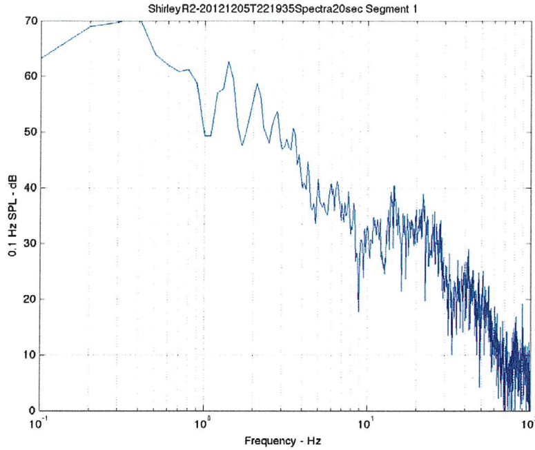
Figure 7. Short (20 sec) duration spectrum with best defined turbine blade harmonics, multiples of 0.7 Hz. Overall SPL of the Blade Pass Signal is 70 dB.
