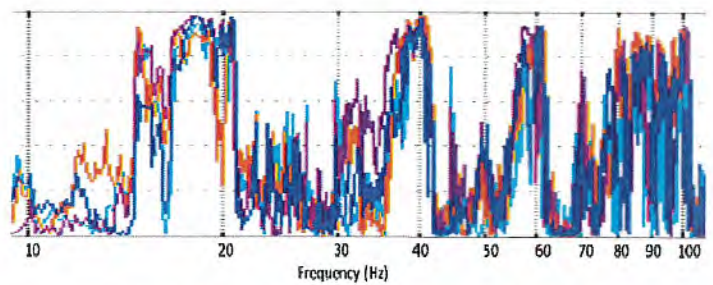
Figure 3a, b: R2-5T204657; Living Room-Blue, Upstairs Bed Room- Orange, Family Room- Turquoise, Basement-Purple, b is an expanded view from 10 Hz to 100 Hz. Note the strong coherence from 20 through at least 80 Hz that resulted from a nearby Helicopter.
