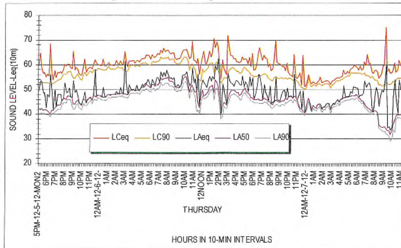
Figure 3.2 Monitor 2 Results
