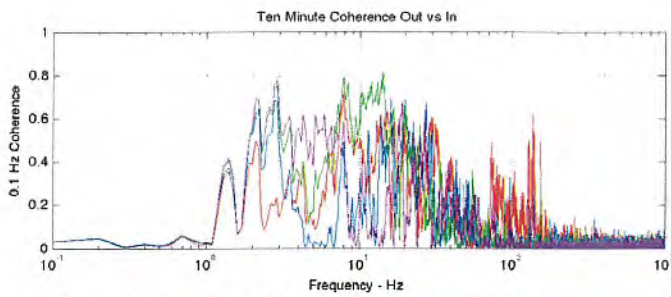
Figure 2a, b: R2-5T204657--coherence with outdoor, ground-plane microphone; Living Room-Blue, Master Bed Room-Red, Behind Kitchen- Green, Basement-Purple, b is an expanded view from 9 Hz to 35 Hz
