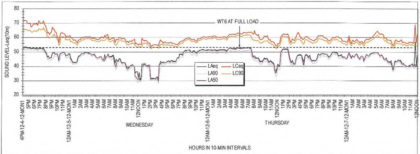
Figure 3.1 Monitor 1 Results
