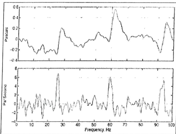
Figure 8. Example ensemble average waveform and time derivative with wind direction 60° re mic orientation.
