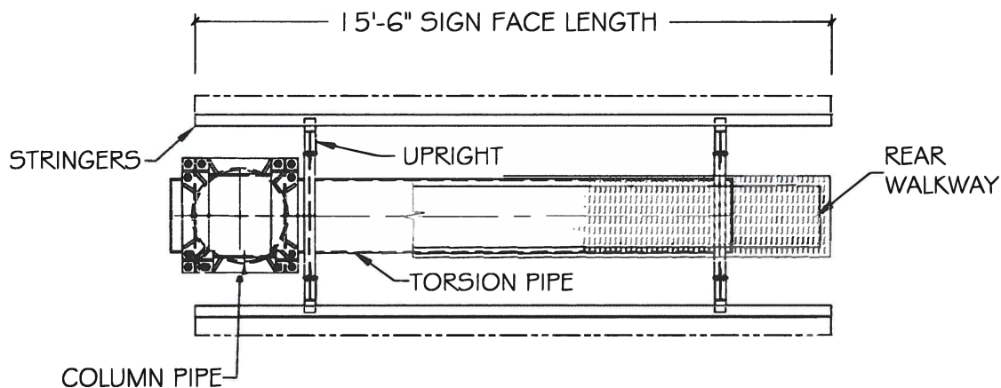
PLAN VIEW
