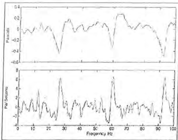
Figure 7. Example ensemble average waveform and time derivative with wind direction 140° to mic orientation.
