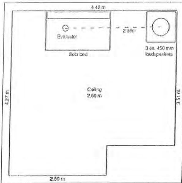
Figure 11. Layout of WTIS evaluation test room.
