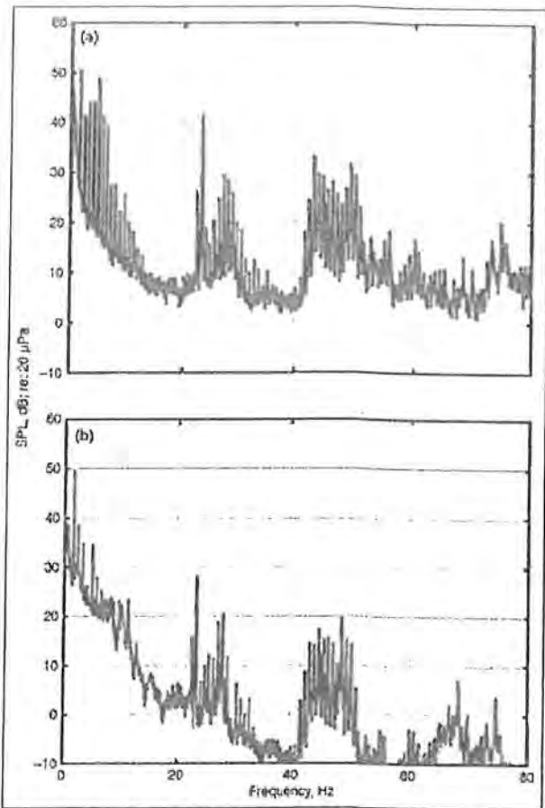
Figure 13. Outdoor (a) and indoor (b) spectra of WTN measured by Hansen.
