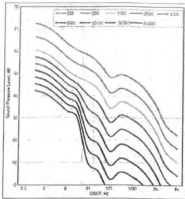
Figure 18. Calculated L_p spectra as function of distance.
