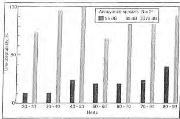
Figure 4. Unacceptability ratings for group of "specials" to noise stimuli.
