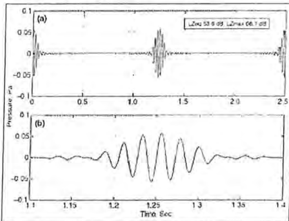
Figure 16. Wave-packet representation of third-spectrum lobe components.
