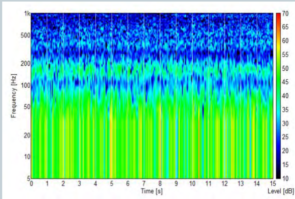
Spectrogram of WTN at Shirley Wind Project, Brown County, Wisconsin (James & Bray, 2010).
