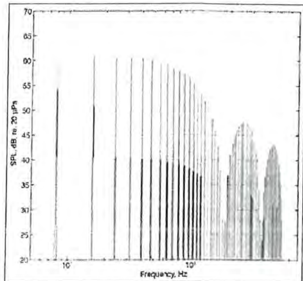
Figure 14. Spectrum of \sin(x)/x -weighted BPF harmonics.
