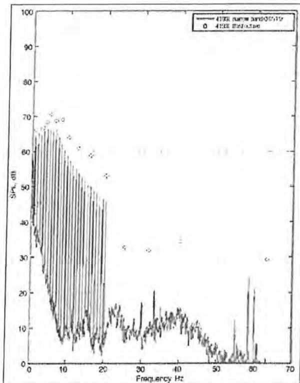
Figure 12. Generic WTIS spectrum used for initial evaluations.
