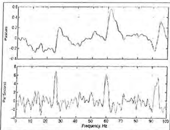
Figure 8. Example ensemble average waveform and time derivative with wind direction 60° to mic orientation.
