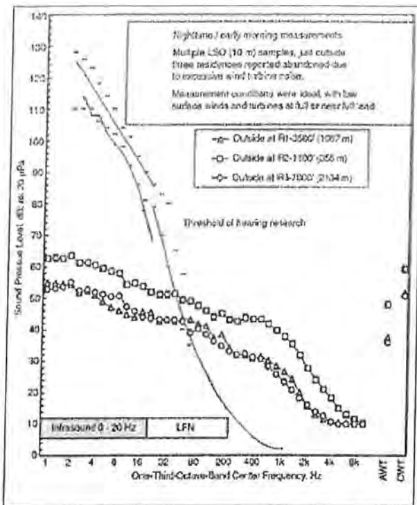
Figure 2. Typical wind turbine spectrum and levels compared to threshold of hearing at low frequencies.
