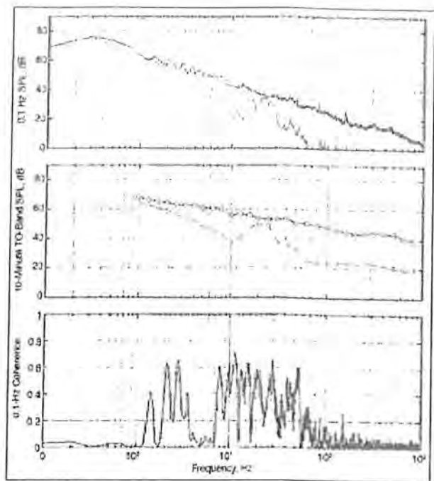
Figure 6. Example of field measurement data.
