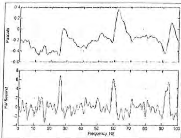
Figure 9. Shaft-order spectrum for wave shown in Figure 8.
