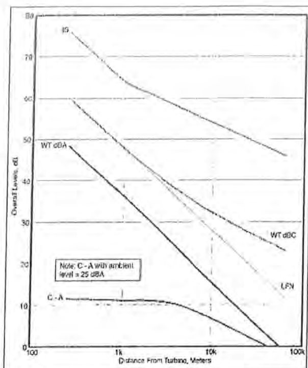
Figure 19. Overall levels as function of distance.
