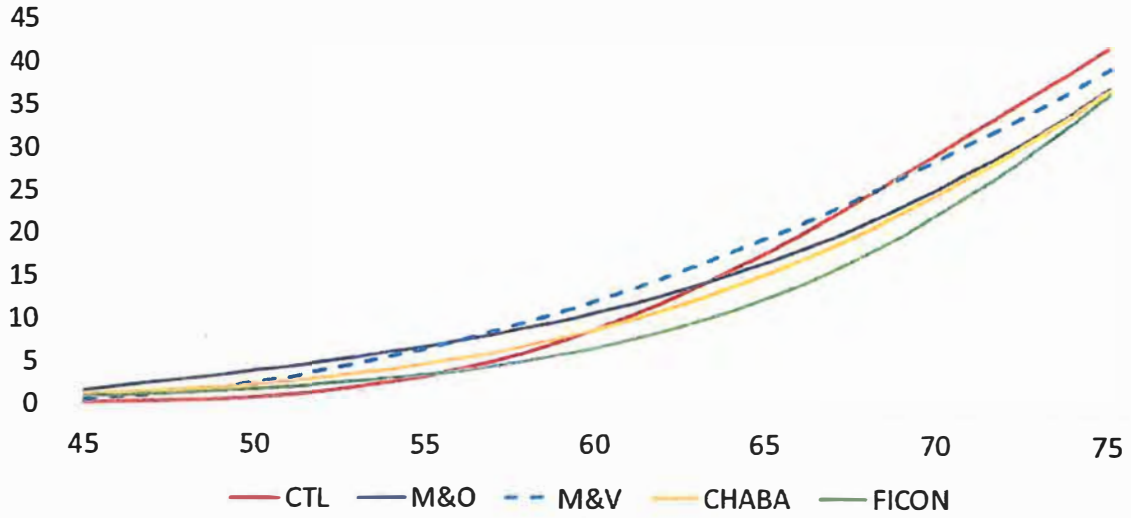
Figure 2A: 5 curves for determining %HA for road traffic noise
