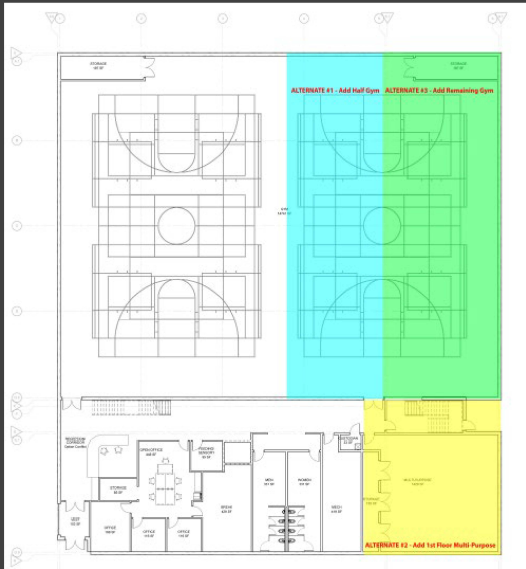
First Floor
